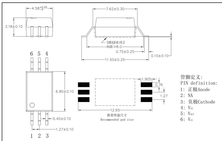
图 22 HGD341W 外形尺寸 Figure 22- The dimensions of HGD341W
