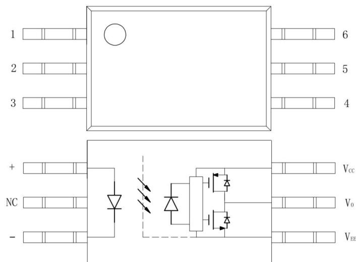
图 2 电原理图 Figure 2-Schematic
