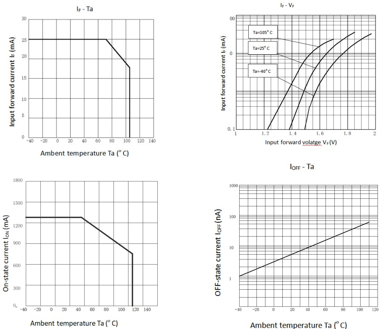
图3 特性曲线 Figure 3- Performance Curves
