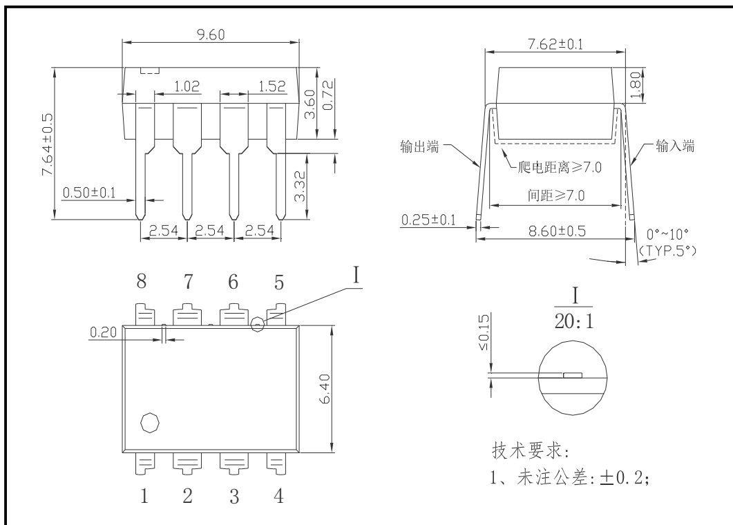
图 3 HSSR-DA05 外形尺寸 Figure 3- The dimensions of HSSR-DA05
