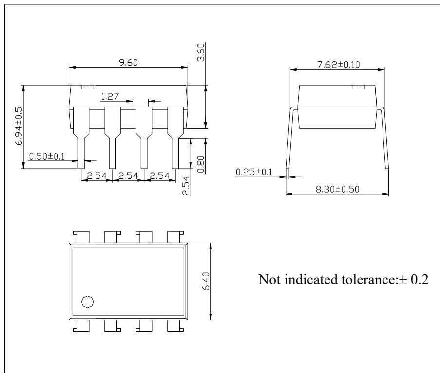
图 4 HGD3120D 外形尺寸 Figure 4- The dimensions of HGD3120D
