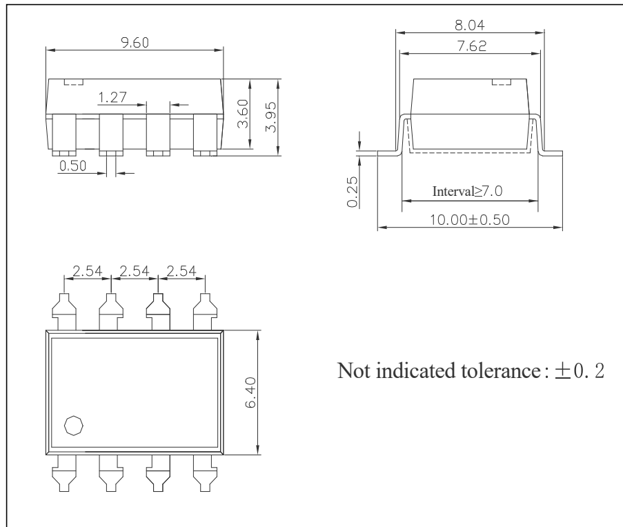
图 5 HGD3120S 外形尺寸 Figure 5- The dimensions of HGD3120S
