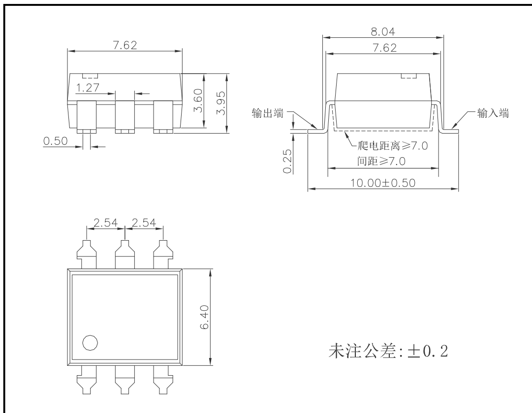
图 5 HSSR-61A08-2 外形尺寸 Figure 5- The dimensions of HSSR-61A08-2
