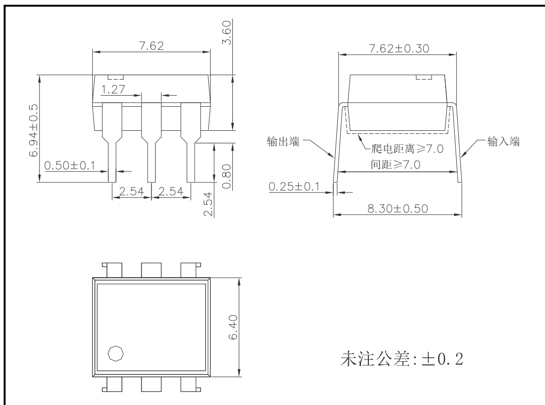
图 3 HSSR-61A08 外形尺寸 Figure 3- The dimensions of HSSR-61A08
