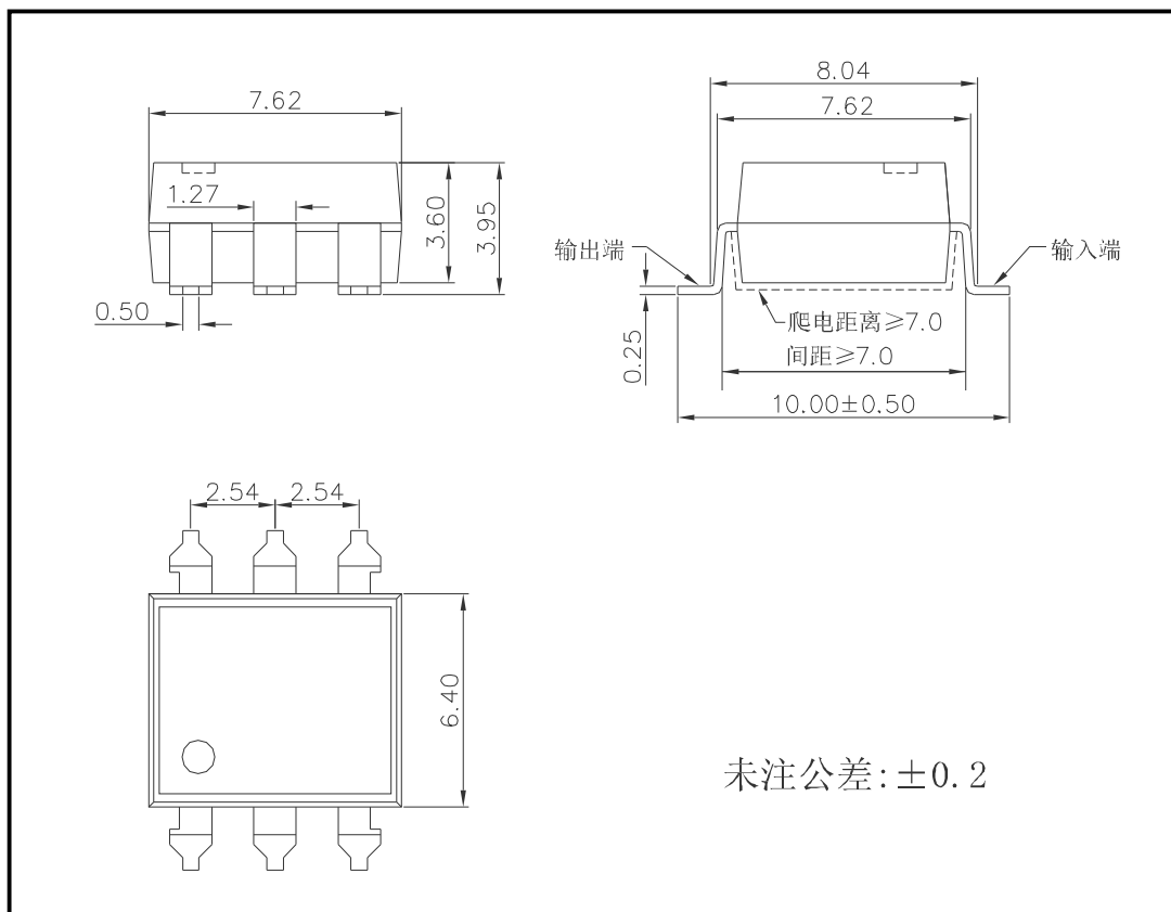
图 5 HSSR-61A06-2 外形尺寸 Figure 5- The dimensions of HSSR-61A06-2
