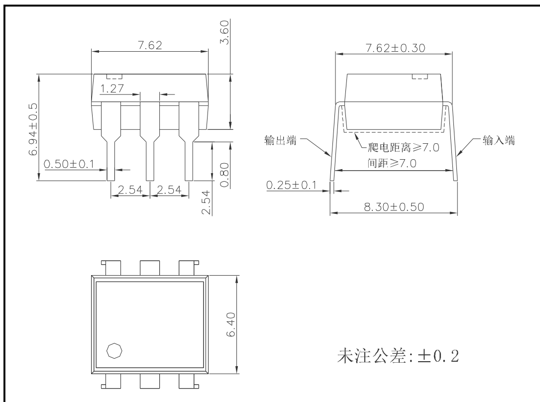
图 3 HSSR-61A06 外形尺寸 Figure 3- The dimensions of HSSR-61A06
