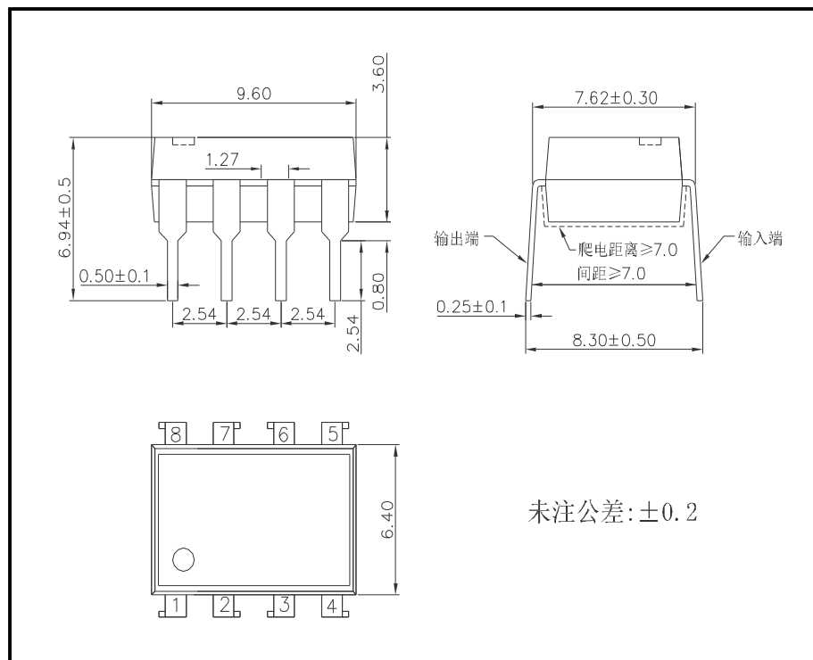
图 3 HSSR-DA08 外形尺寸 Figure 3- The dimensions of HSSR-DA08
