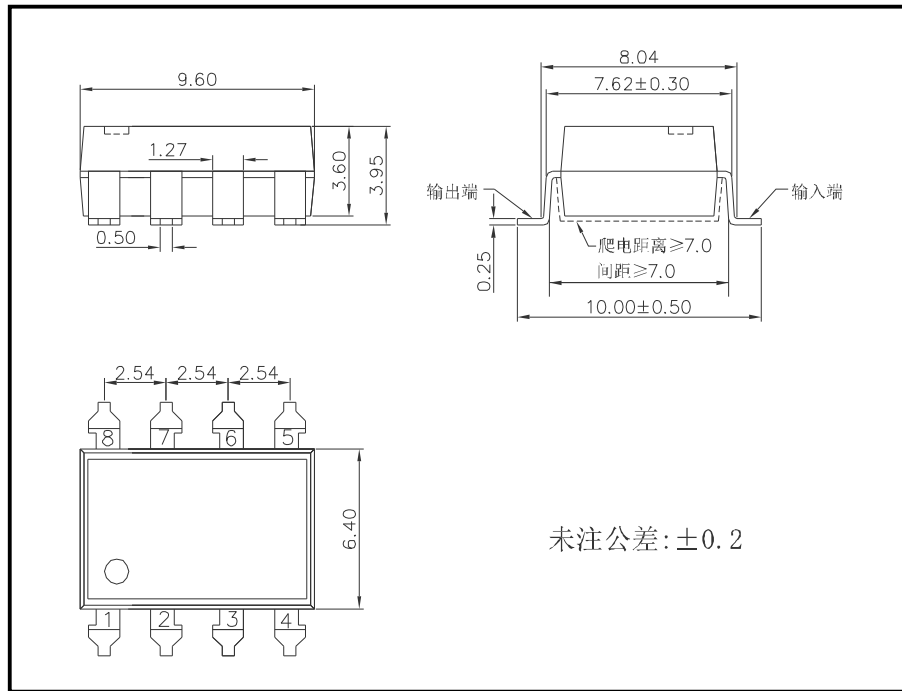
图 4 HSSR-DA08-2 外形尺寸 Figure 4- The dimensions of HSSR-DA08-2
