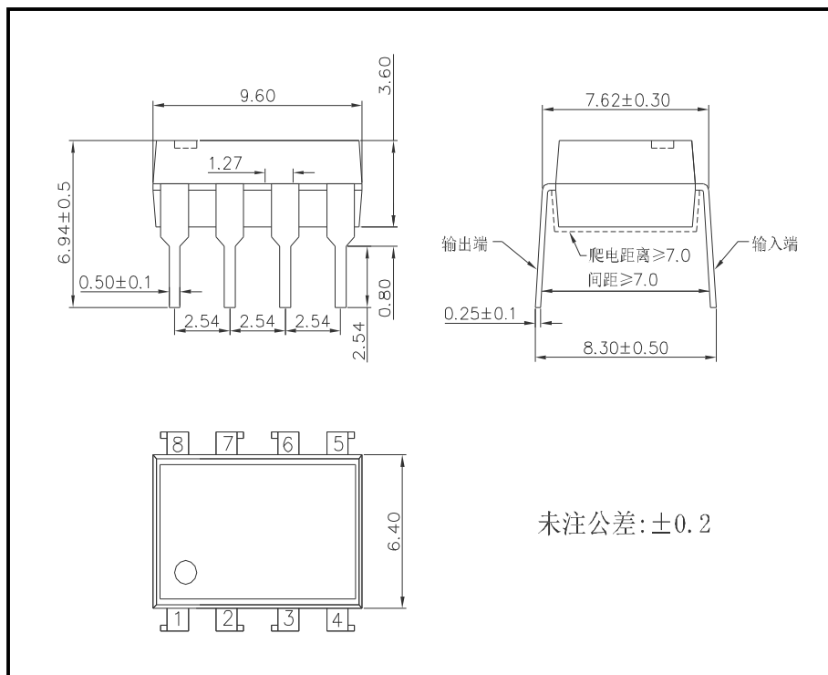
图 3 HSSR-DA06 外形尺寸 Figure 3- The dimensions of HSSR-DA06
