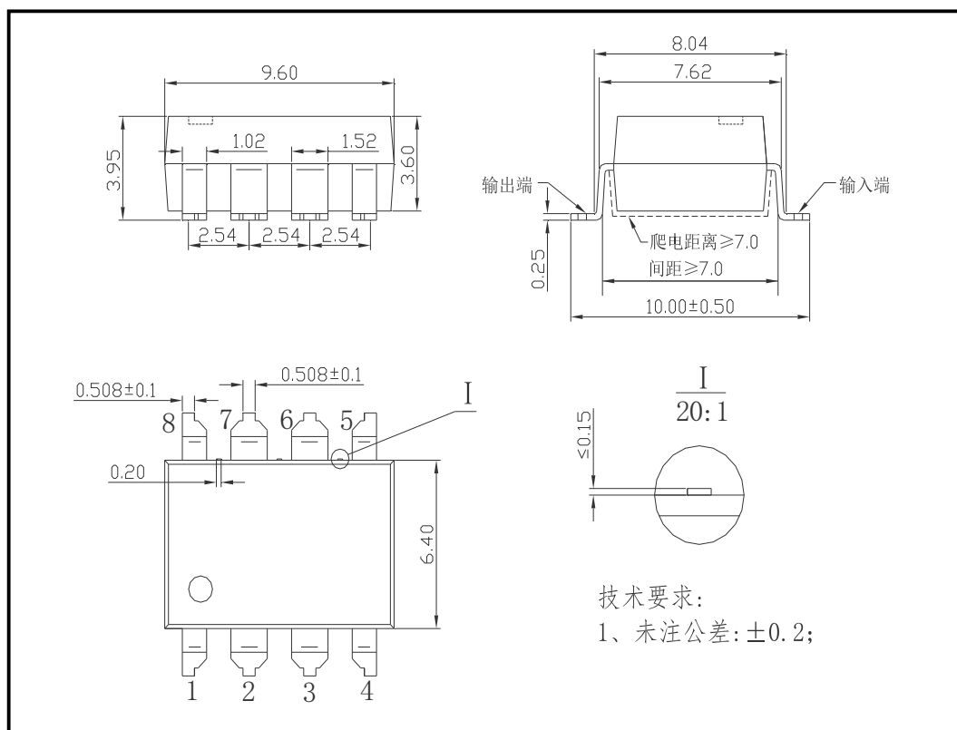
图 4 HSSR-DA04-2 外形尺寸 Figure 4- The dimensions of HSSR-DA04-2
