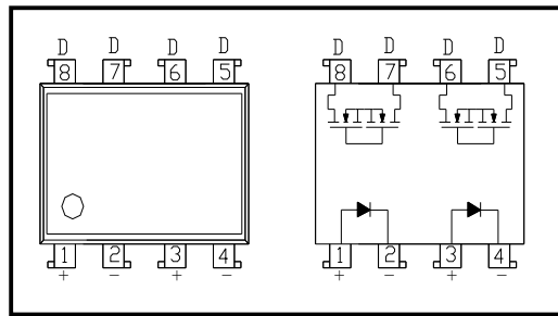
图 2 电原理图 Figure 2-Schematic
