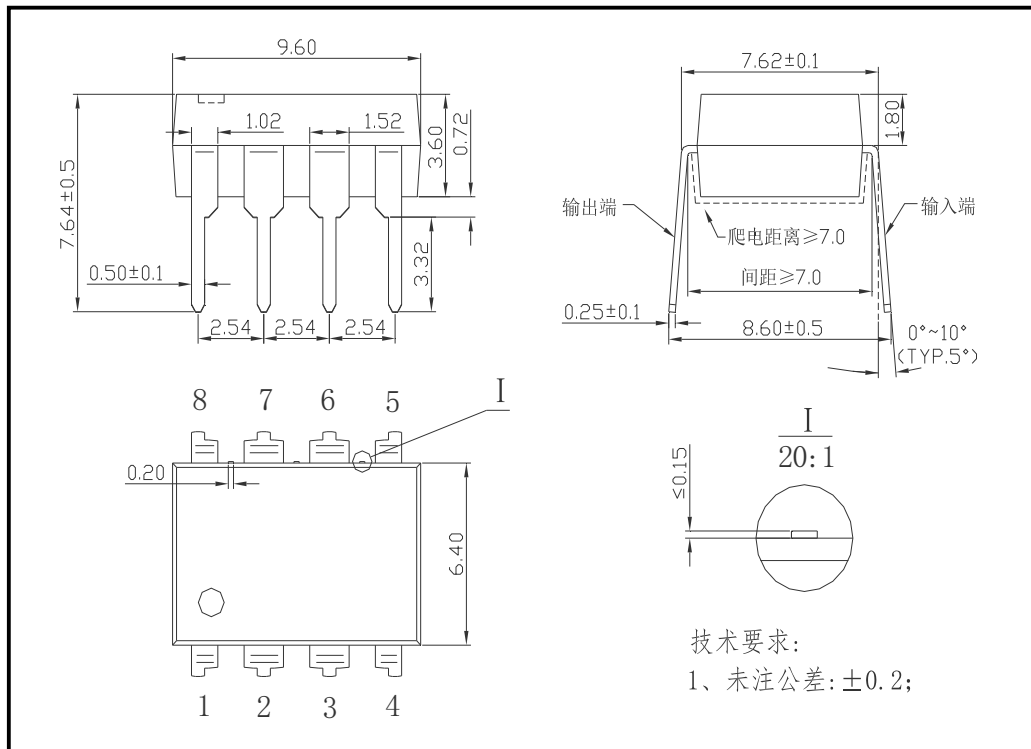
图 3 HSSR-DA04 外形尺寸 Figure 3- The dimensions of HSSR-DA04
