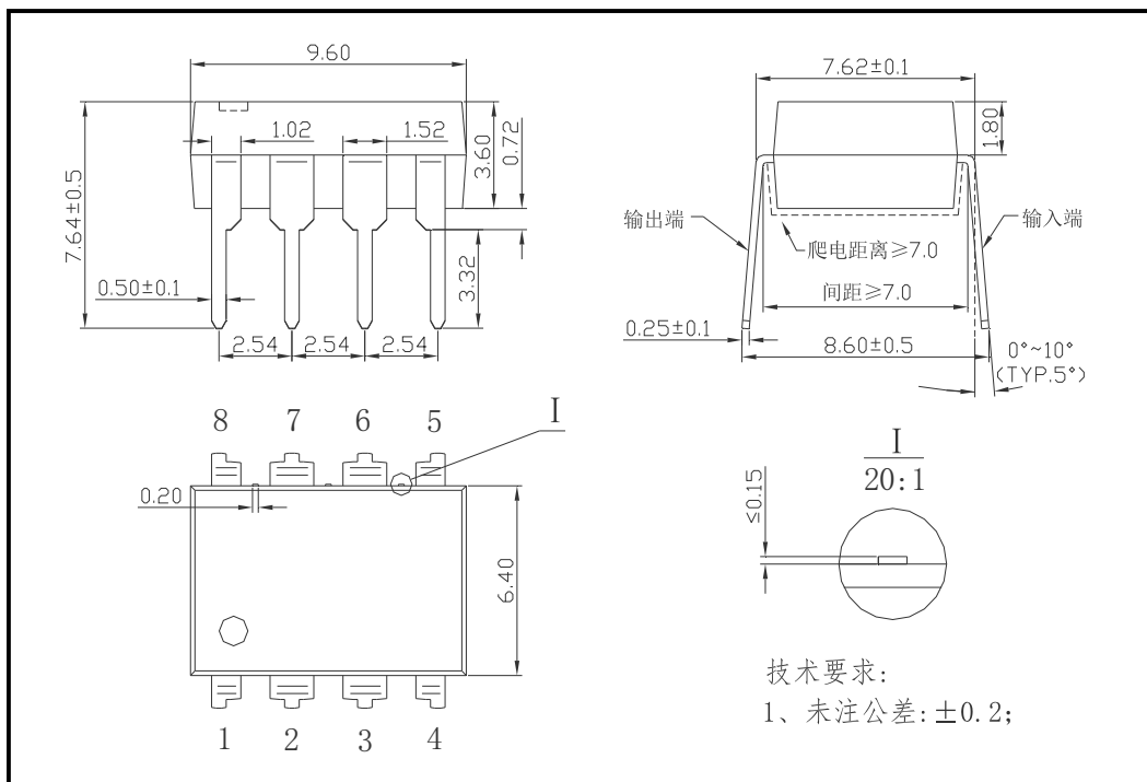
图 3 HSSR-DA01 外形尺寸 Figure 3- The dimensions of HSSR-DA001
