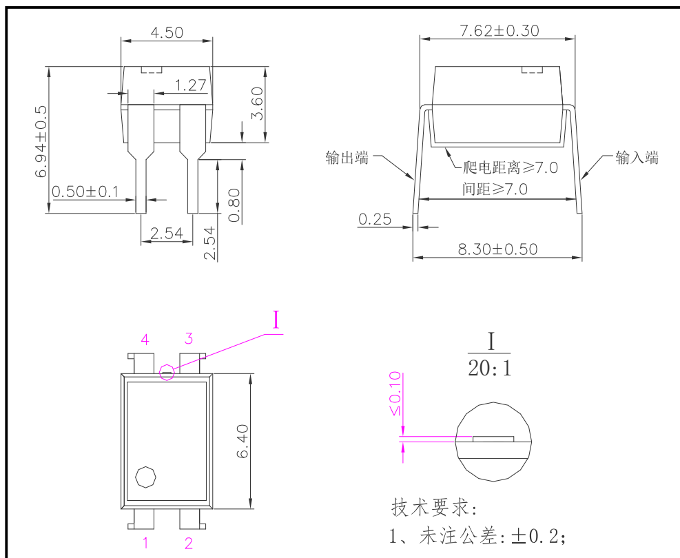
图 3 HSSR-41A06 外形尺寸 Figure 3- The dimensions of HSSR-41A06
