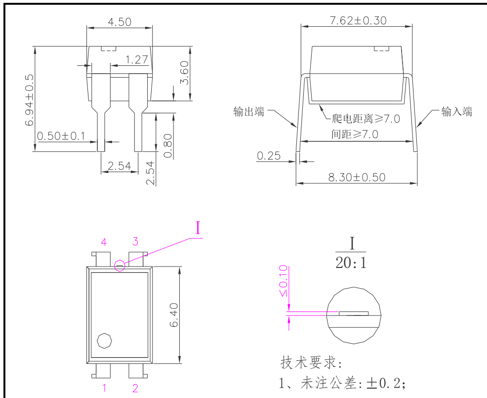
图 3 HSSR-41A04 外形尺寸 Figure 3- The dimensions of HSSR-41A04
