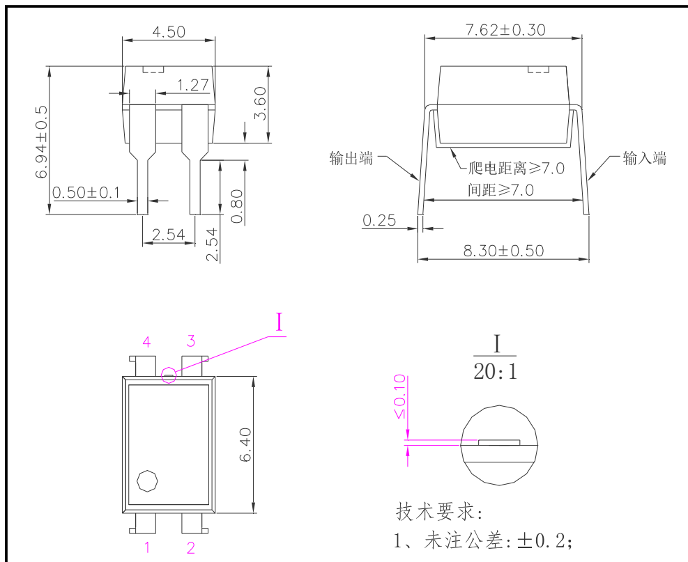
图 3 HSSR-41A01 外形尺寸 Figure 3- The dimensions of HSSR-41A01
