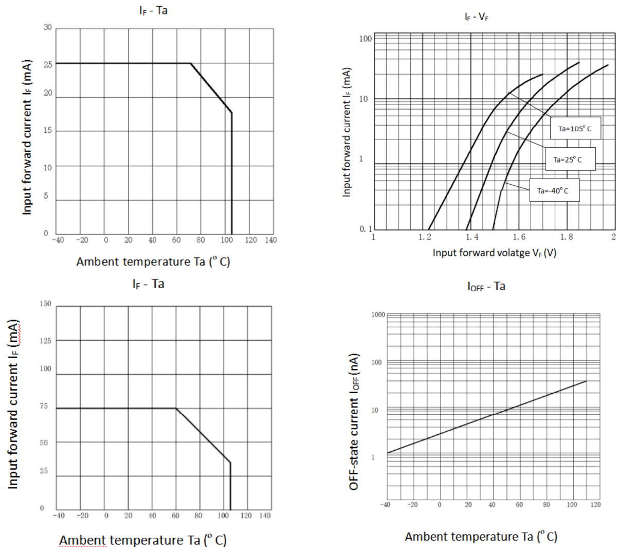
图 3 特性曲线 Figure 3- Performance Curves
