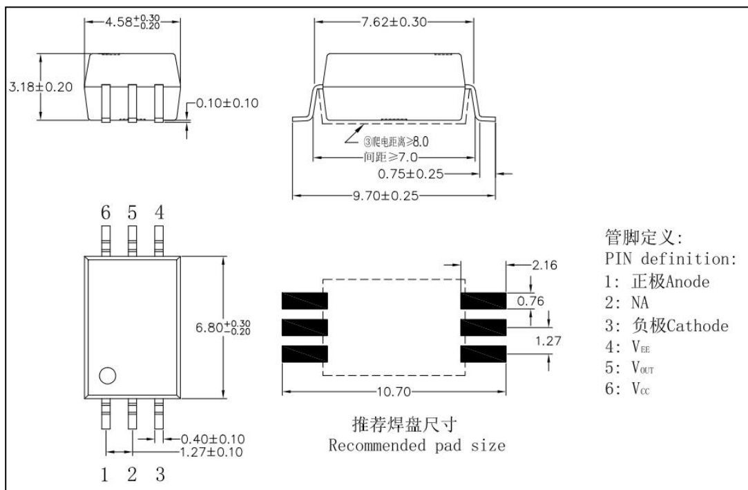
图 22 HGD341P 外形尺寸 Figure 22- The dimensions of HGD341P
