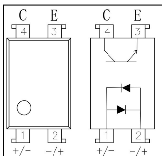
图 2 电原理图 Figure 2-Schematic
